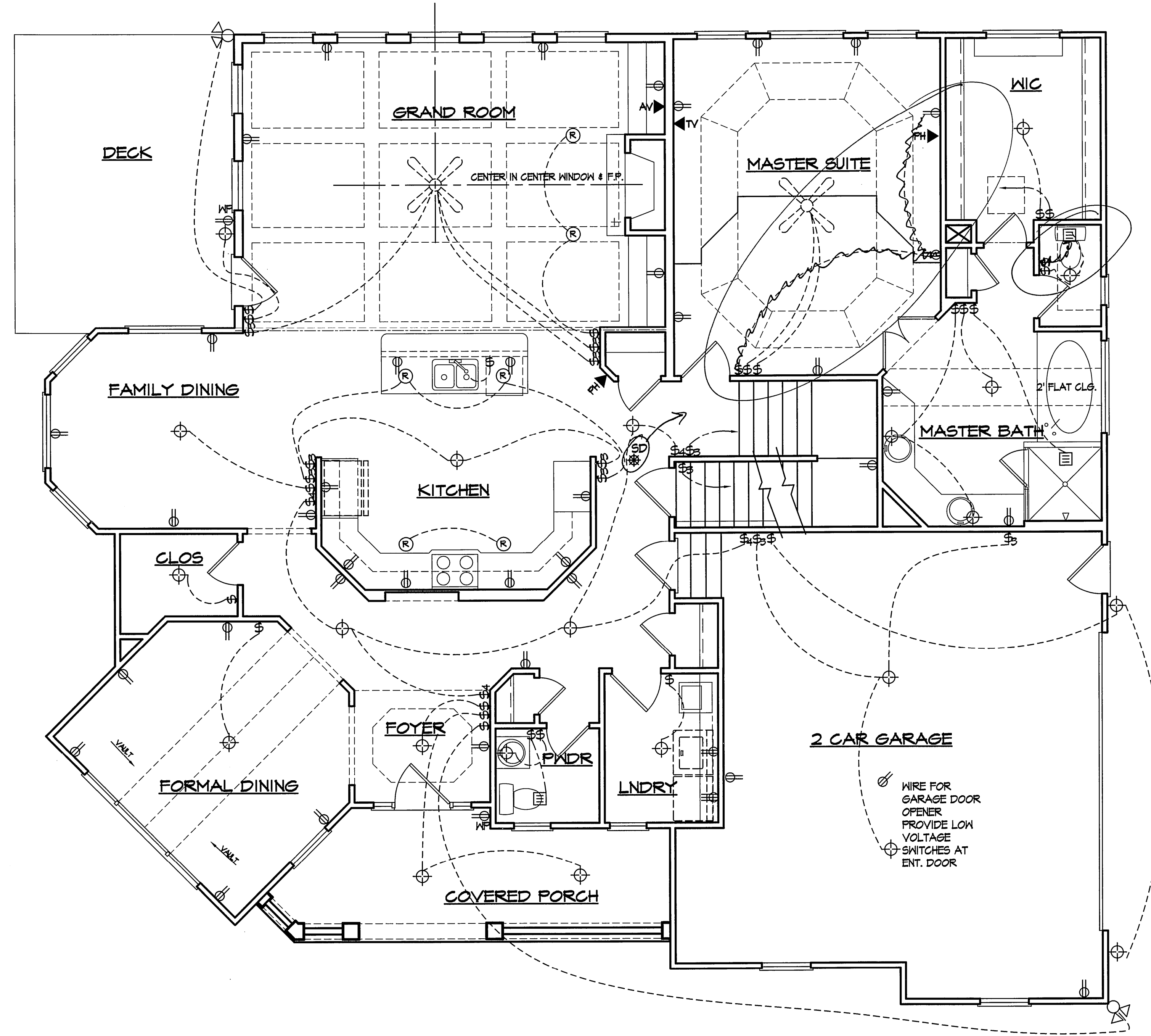
MAIN LEVEL ELECTRICAL PLAN SCALE: 1/4" = 1'-0"
